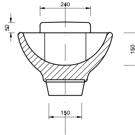
SECTIONAL FRONT VIEW
