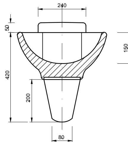
SECTIONAL FRONT VIEW
